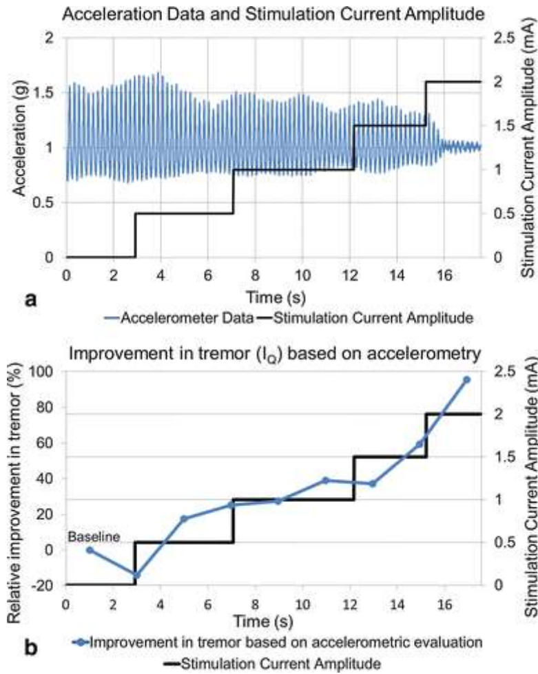
Figure 2. a Raw acceleration data (blue signal) recorded in synchronization with the stimulation amplitude (black stepped line). b Improvement in tremor estimated from the outcome measures extracted from accelerometer data ( I_Q ) for the different stimulation current amplitudes (color figure online).
